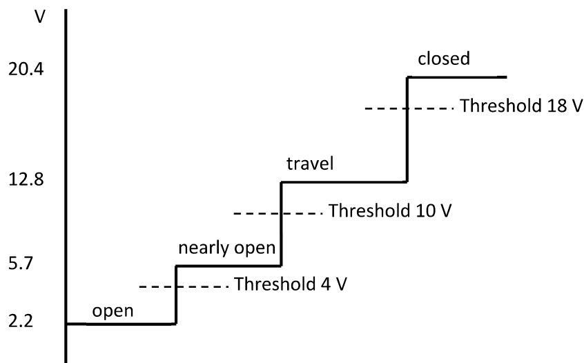
Figure 9 Voltage Input with Limit Switch Position
