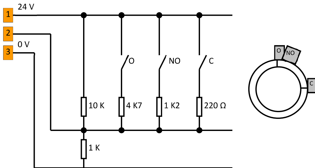
Figure 8 Position Limit Switches and circuit
