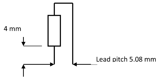
Figure 12 Resistor Forming
