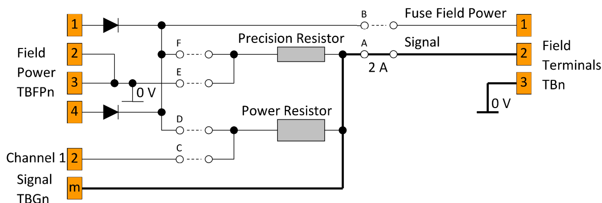
Figure 5 Digital Outputs
