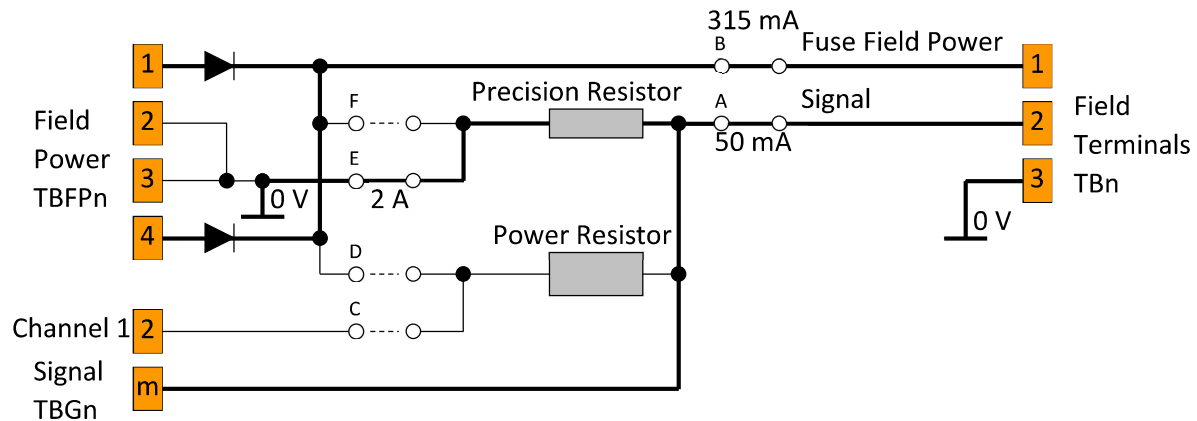
Figure 6 Current Sourcing Analogue Inputs
